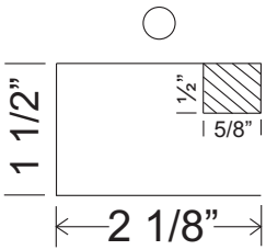
Back Top Notch Right Side (as shown)
