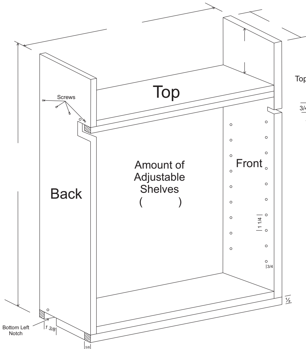
Back Top Notch Right Side (as shown)
